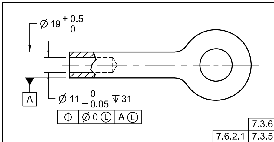
Fig. 7-17 Datum Feature at LMB
