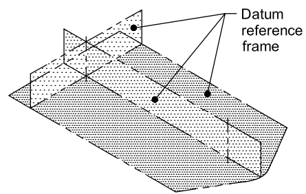
(e) Datum reference frame
