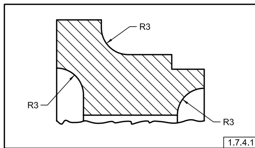
Fig. 1-15 Leader-Directed Dimensions
