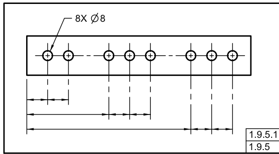
Fig. 1-54 Repetitive Features
