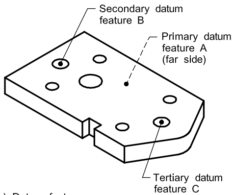
(b) Datum features
